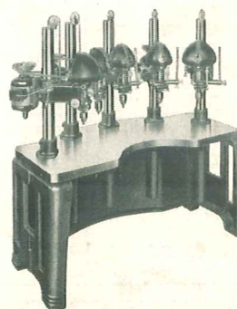
Special Production Set-up made of standard 14" heads and accessories.
